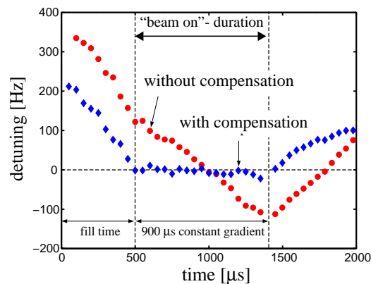
Fig. 5: Demonstration of active Lorentz force compensation with a PZT driven tuner (TTF 9-cell cavity at 23.5 MV/m flat-top gradient).
