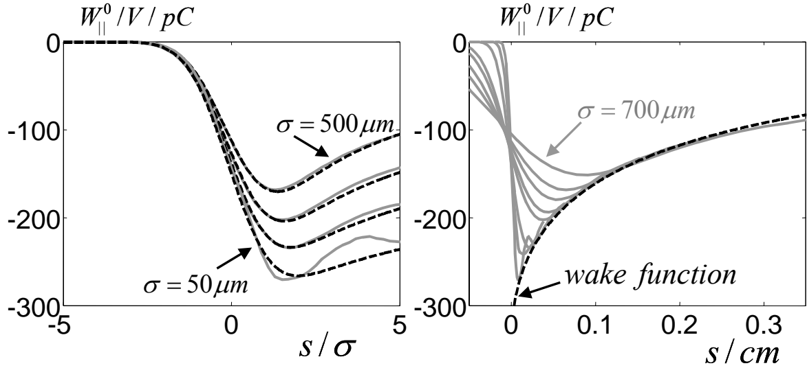
Fig5. Comparison of analytical and numerical longitudinal wake potentials in the third cryomodule ( \sigma = 50 \div 700 \mu\text{m} ).
