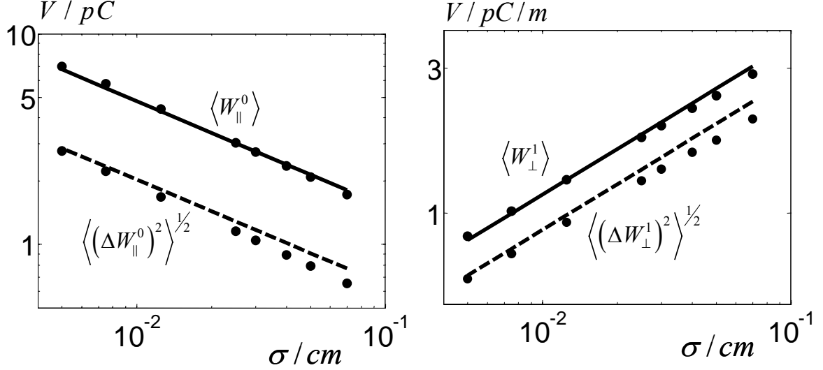
Fig 2. Comparison of numerical and analytical integral parameters for single-cell structure.
