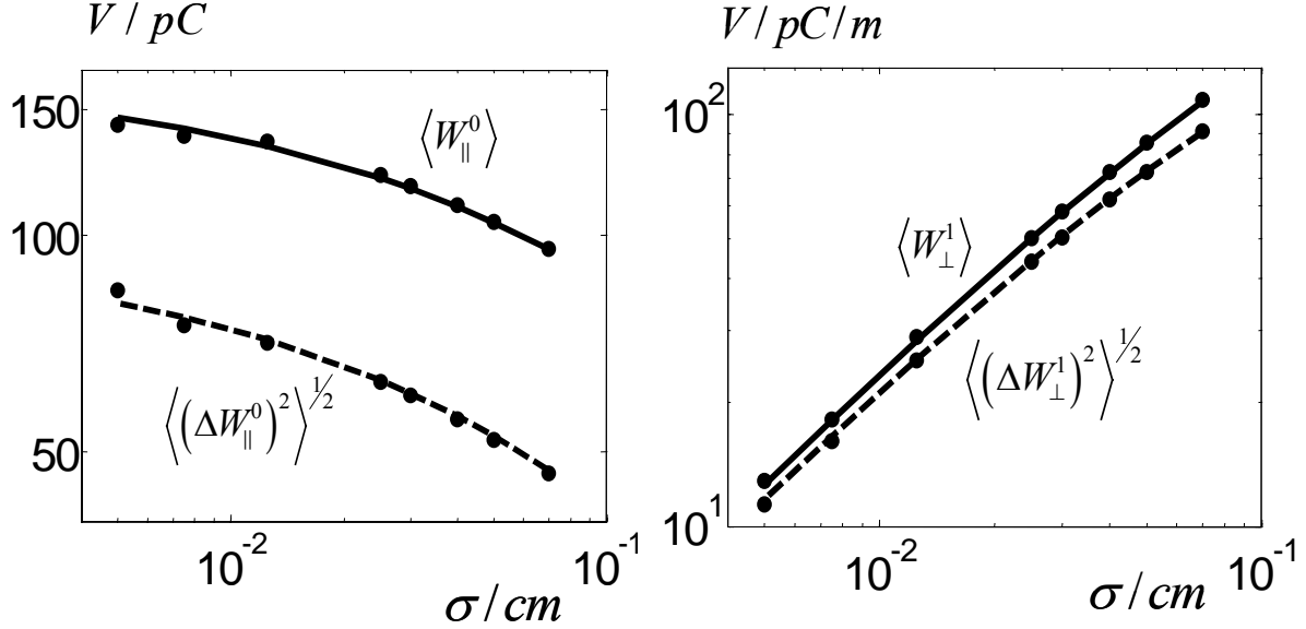
Fig 7. Comparison of numerical and analytical integral parameters for the third TESLA cryomodule.
