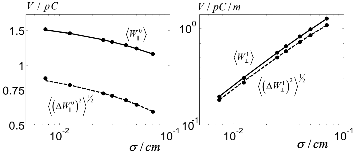
Fig 4. Comparison of numerical and analytical integral parameters for periodic structure.
