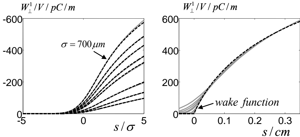
Fig 6. Comparison of analytical and numerical transversal wake potentials in the third cryomodule ( \sigma = 50 \div 700 \mu\text{m} ).
