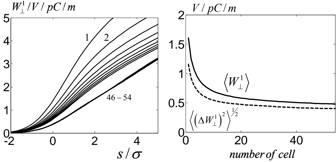
Fig 3. Modification of the transverse wake potentials and the kick factor in periodic structure.
