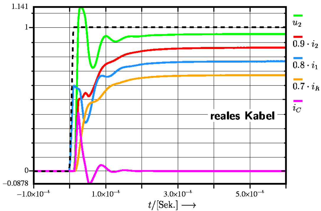
Fig.9: Simulation result of 4 cables 75 mm 2 in parallel 2500 m
