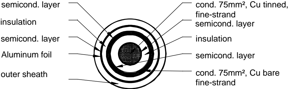
Fig .1: Cross section of the cable
