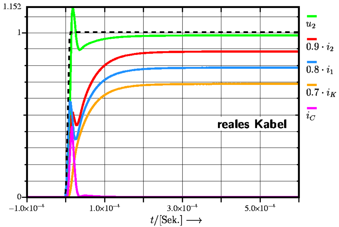
Fig. 8: Simulation result of 4 cables 75 mm 2 in parallel 1000 m
