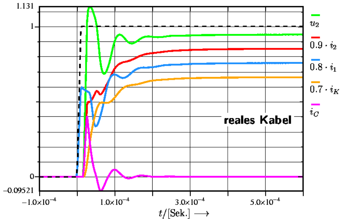
Fig.10: Simulation result of 4 cables 75 mm 2 in parallel 3000 m
