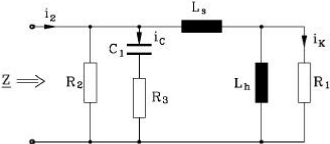
Fig. 6: Impedance matching network
