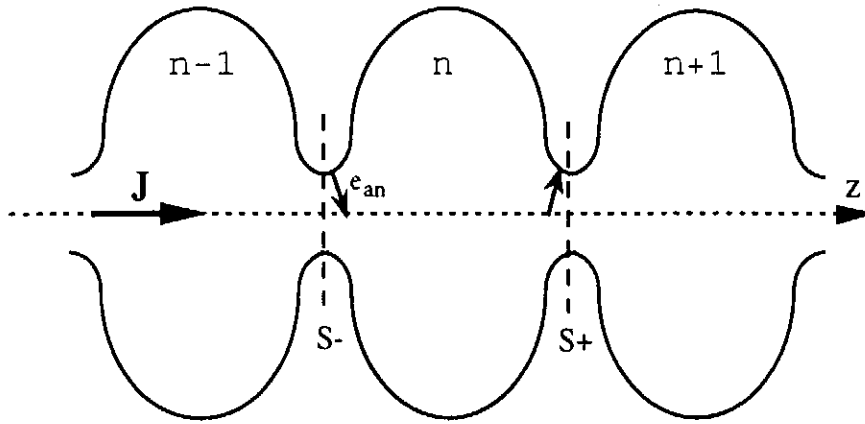
Figure A-1 : Chain of coupled resonant cells
