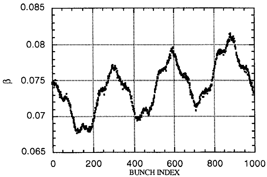
Figure 16: Twiss parameter \beta [m]
