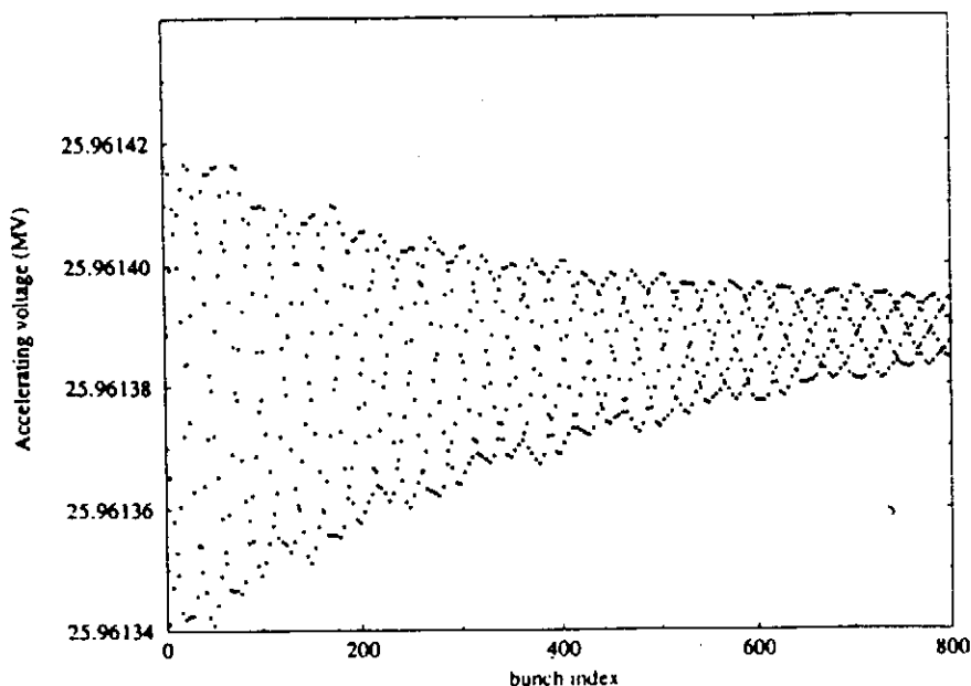
Figure 4 : Accelerating voltage evolution during 800 bunches
