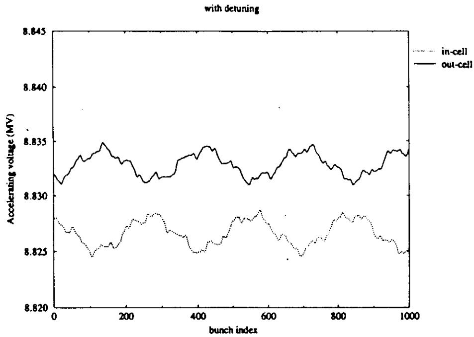
Figure 8 : Energy gain evolution with cavity detuning.
