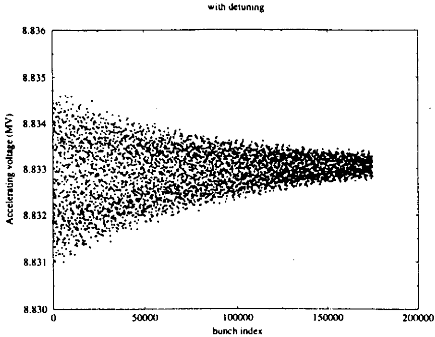
Figure 10 : Energy gain evolution on a longer time-scale (with cavity detuning).
