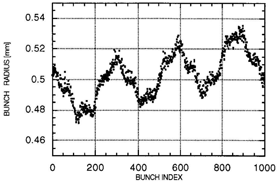
Figure 13: Bunch Radius [mm]
