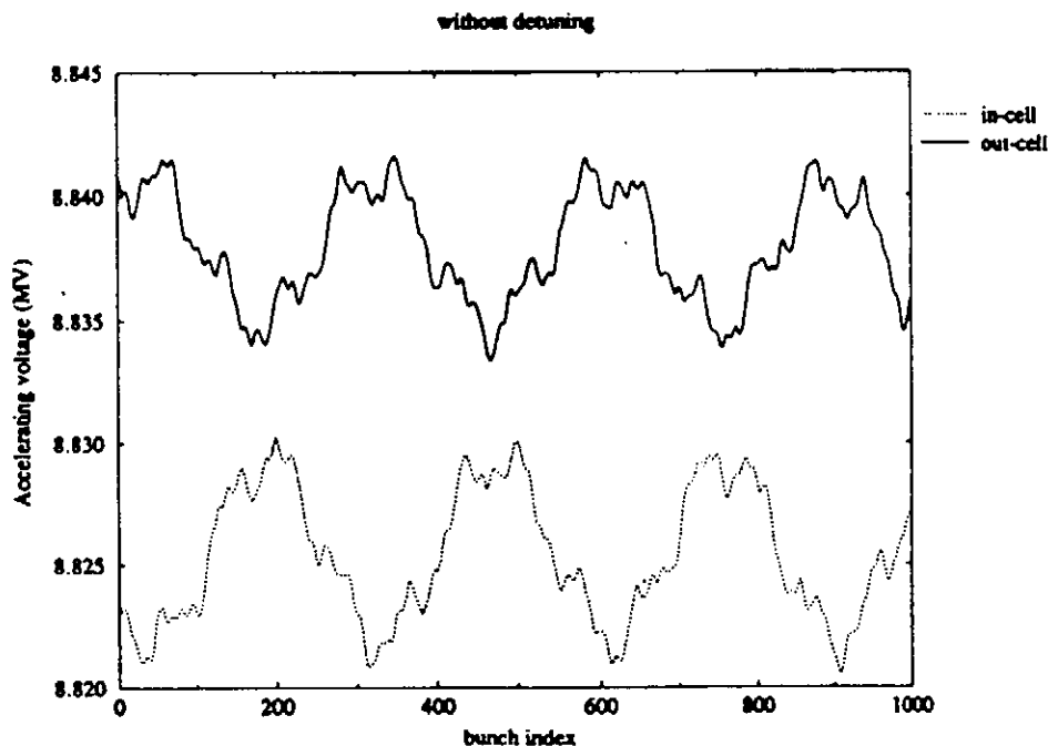
Figure 7 : Energy gain evolution without cavity detuning
