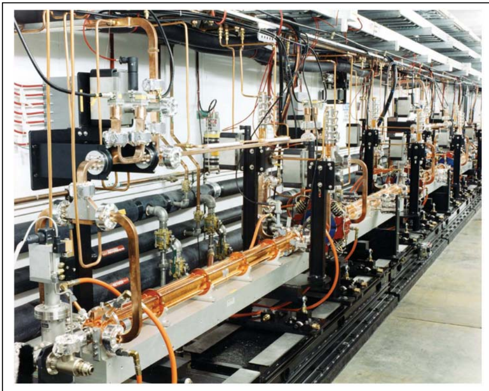
FIGURE 3. High Field Test Stand at NLCTA of SLAC. This picture was taken from [16].
