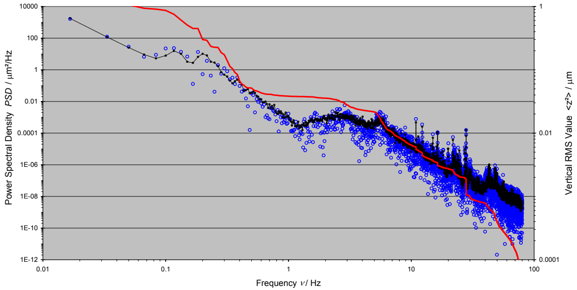
Figure 5: Vertical power spectral density (open points) and root mean square value (thick line) calculated from a one minute data file taken at 12:00 h on December 9, 2004. The thin line with the filled points is the average over 15 minutes of the PSD.
