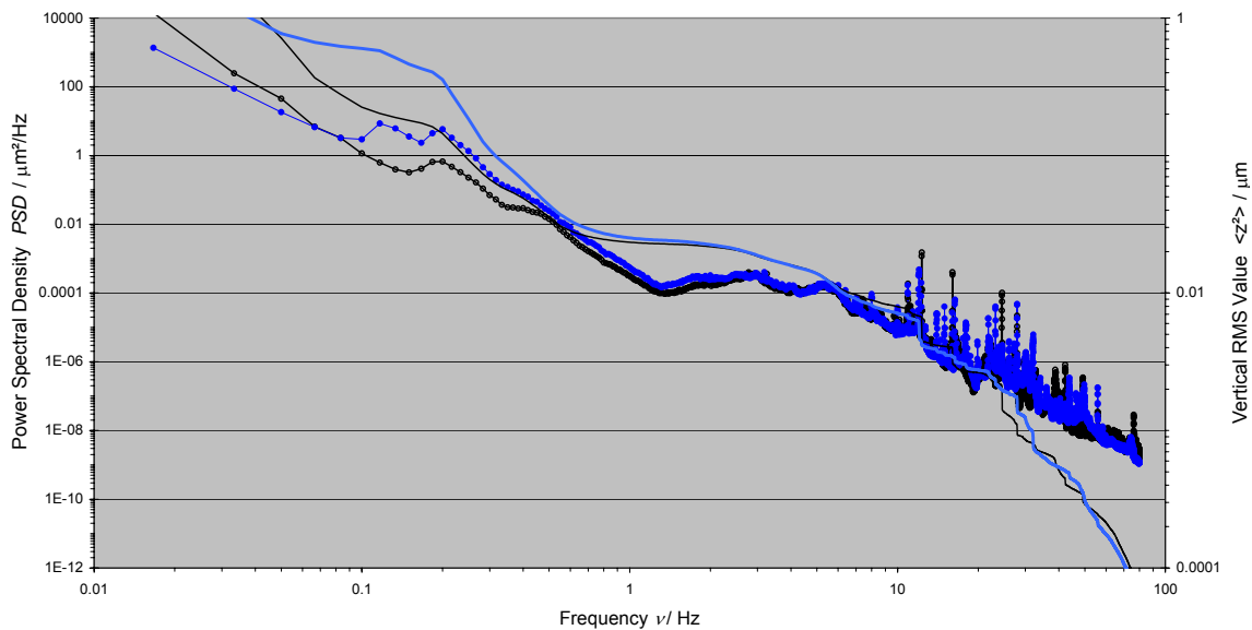
Figure 11: Comparison of the power spectral density (lines with points) and RMS values (lines), averaged over 17 hours, taken in August and in December.
