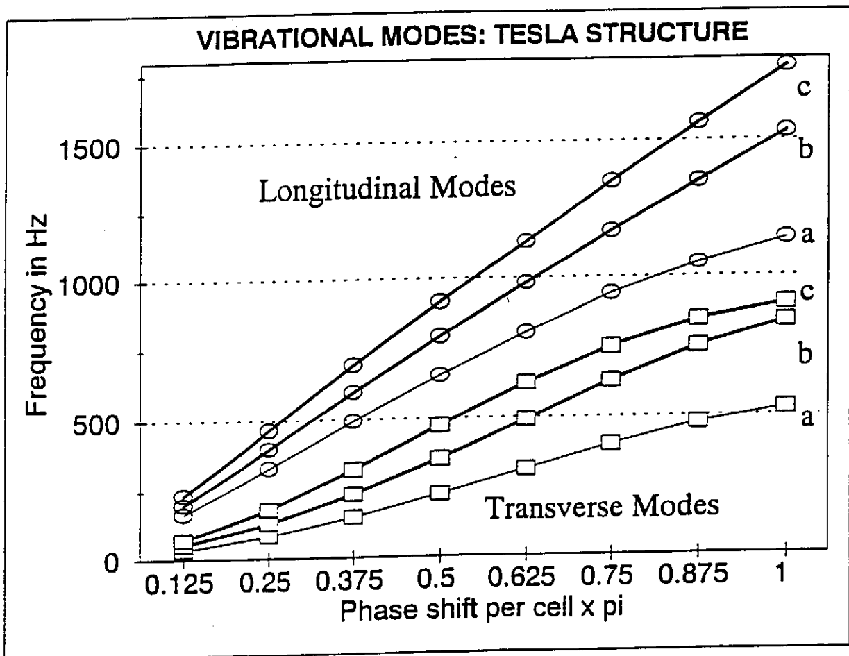
Figure 2. Vibrational modes of the TESLA structure: a) the bare structure, b) the structure with annular stiffeners, c) the structure (with stiffeners) constrained by a rigid helium vessel.
