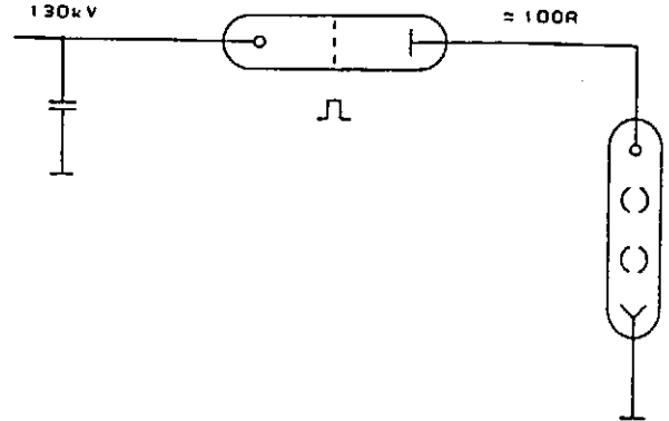
Fig. 3: Klystron modulator with a series switch tube.
