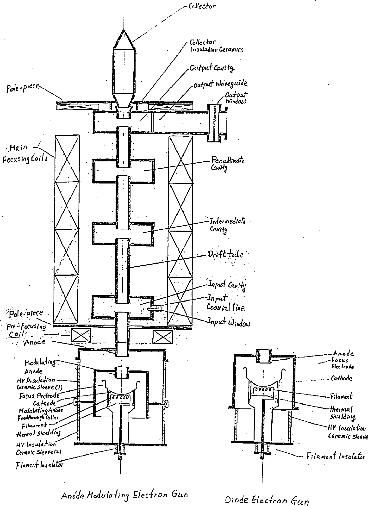
Fig. 1: Klystron with and without modulating anode.
