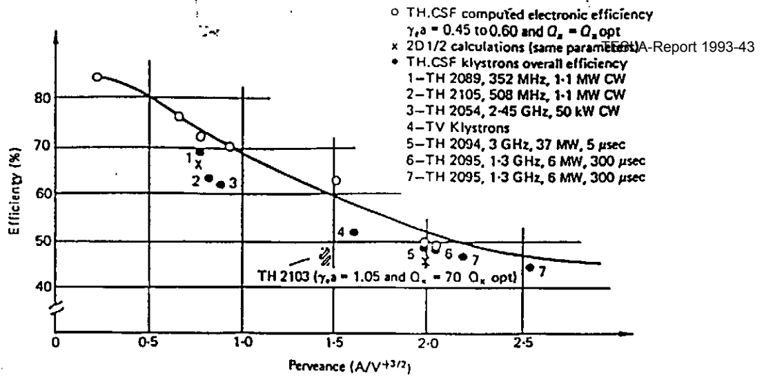
Fig. 12: ( Taken from ref. 7) Influence of Perveance on Klystron efficiency.
