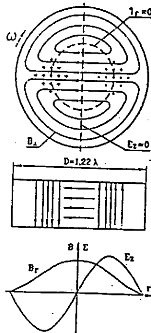
Fig. 15: ( Taken from ref. 8) Distribution of electromagnetic fields in magnicon cavities.
