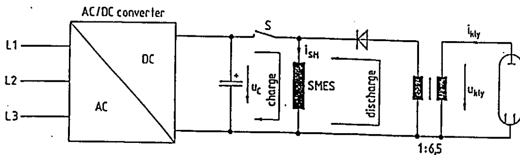
Fig. 4: Schematic electrical circuit of the Superconducting Magnetic Energy Storage (SMES) coil circuit coupled to a Klystron through a pulse transformer. Transfer of a part of the electrical energy stored in the superconducting coil requires switching of the high current in the coil at a 10 Hz rate. An appropriate switch and superconducting cable suitable for a dB/dt of 20 T/s corresponding to a pulse current droop of 2 % within 2 ms need to be developed.
