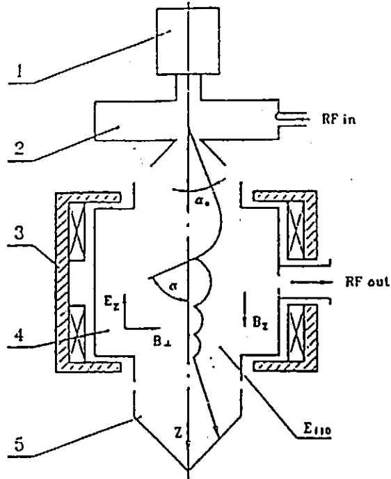
Fig. 14: ( Taken from ref. 8) Schematic of the magnicon: 1—source of electrons; 2—circular deflection cavity; 3—solenoid; 4—output cavity; 5—collector.
