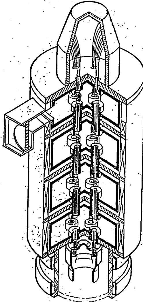
Fig. 13: ( Taken from ref. 7) Structure of Multibeam Klystron
