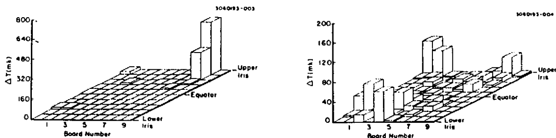
(a). E_{peak} = 31 MV/m; 1st CW power rise. (b). E_{peak} = 36 MV/m; final CW power rise Figure 8. Temperature maps from the test of cavity 1-5.
