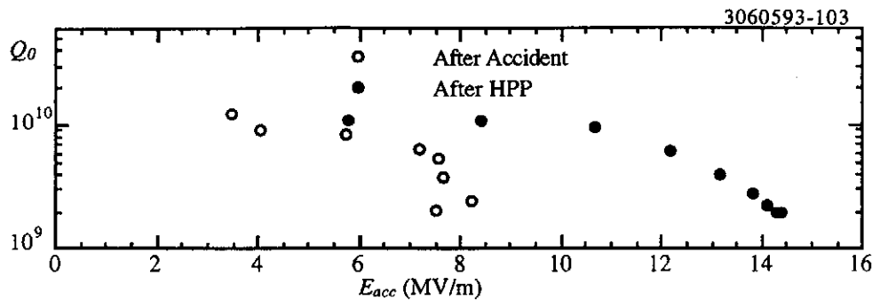
Figure 6. Q_0 vs. E_{acc} plots showing nine-cell cavity behavior before from the second vacuum accident.
