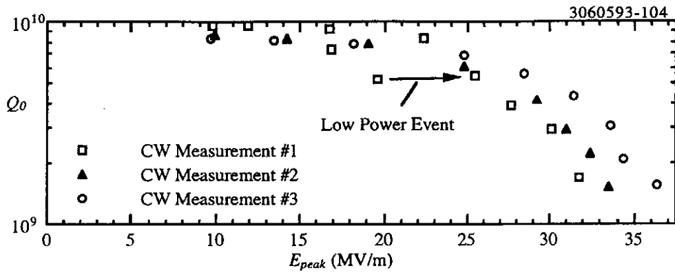
Figure 7. Q_0 vs. E_{peak} curves from low power measurements on single-cell cavity 1-5.
