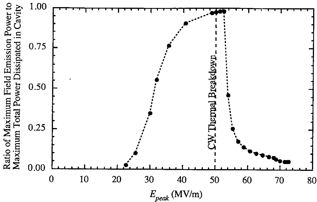
Figure 18. The ratio of maximum power coupled into field emission to the maximum power dissipated in the cavity (both simulated via the program described in the text), plotted as a function of the maximum peak electric field reached during the RF pulse. For fields less than 25 MV/m, FE is not a significant load on the cavity. As the CW thermal breakdown limit is surpassed, the expanding normal conducting region of the RF surface becomes the dominant loss mechanism.
