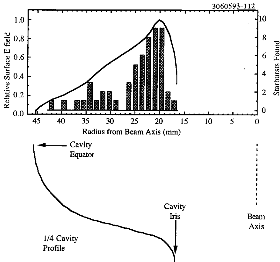
Figure 12. Radial distribution of "Starburst" phenomena found in all examined single-cell cavities, plotted along with relative surface electric field.
