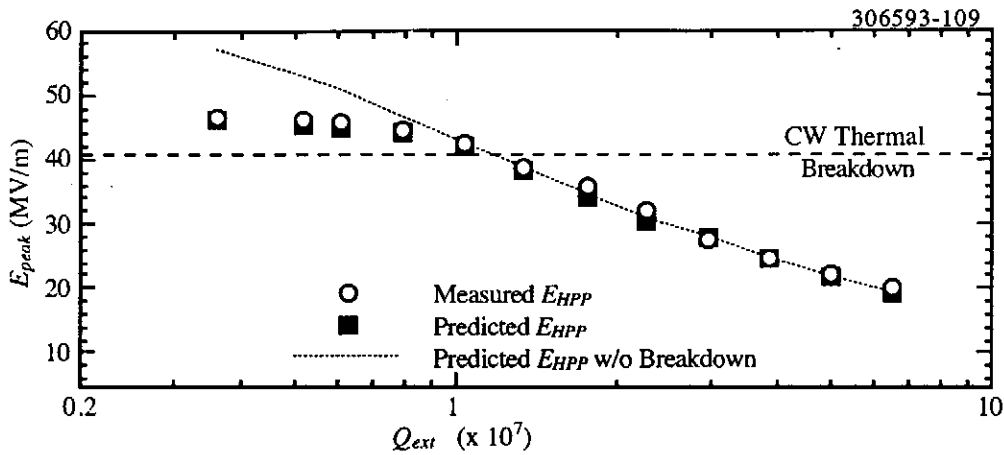
Figure 16. Comparison of Measured and Predicted E_{HPP} during HPP on a nine-cell cavity.
