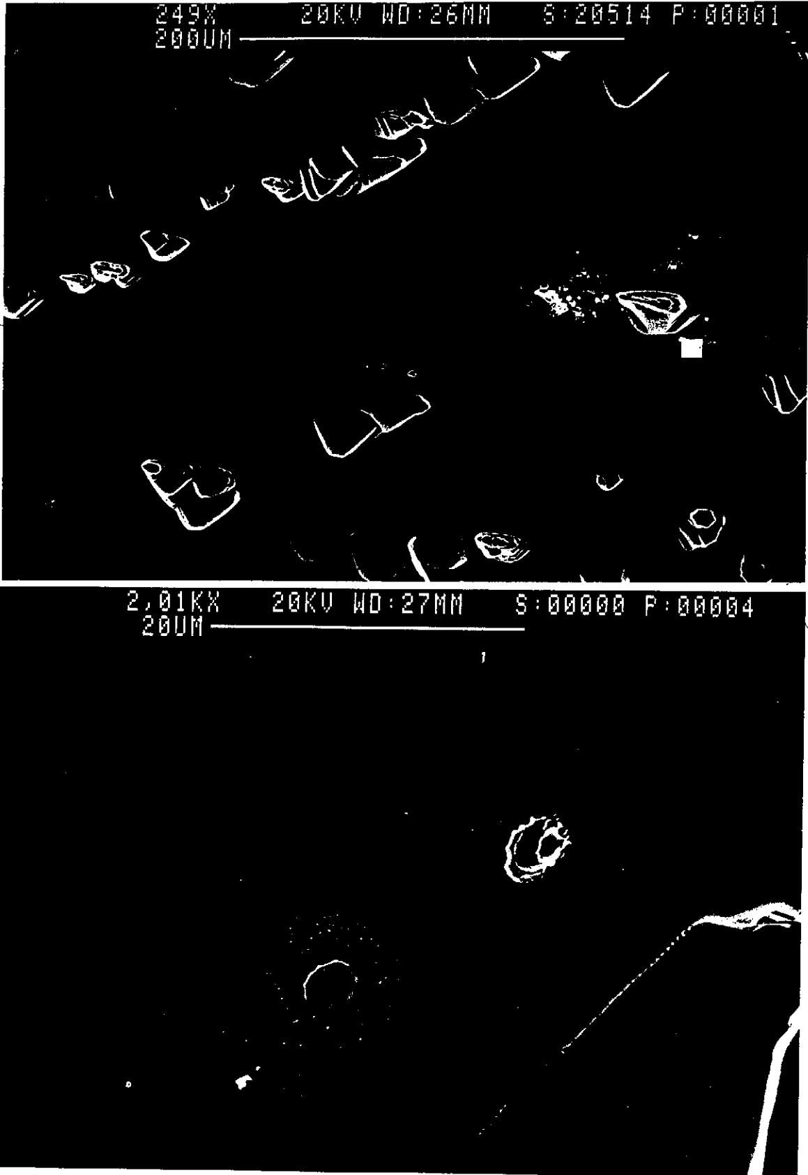
Figure 11. SEM photographs of the starburst region found in cavity 1-5. The starburst and craters are located in a position to explain the processing event. The lower picture is an enlargement of the central region of the top picture. Contaminant materials include Ca, Ti, C, and O.
