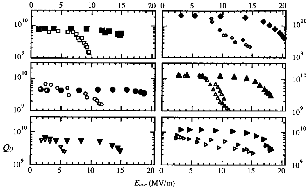
Figure 2. Composite Q_0 vs. E_{acc} plots of the six best tests of nine cell cavities. Open symbols show cavity behavior before processing; closed symbols are for after HPP.
