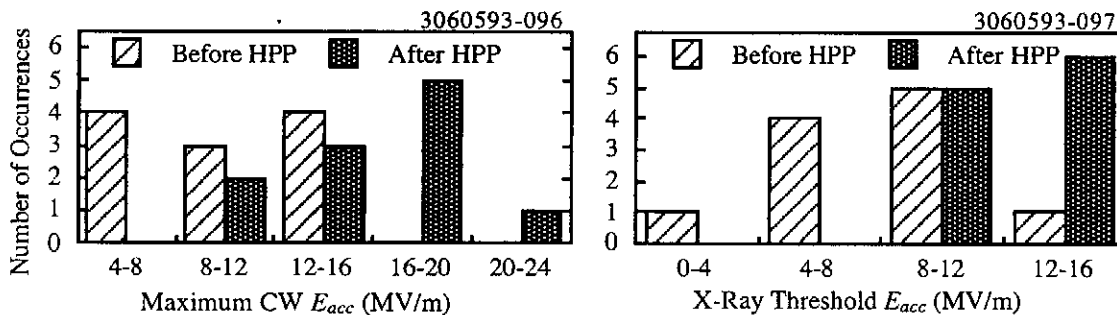
Figure 1. Histogram plots of maximum achieved CW accelerating gradient and X-ray detection threshold accelerating gradient, before and after HPP processing. For the maximum attainable gradient plot: prior to HPP, \langle E_{acc} \rangle = 11.9 MV/m (s.d. = 3.4 MV/m); following HPP, \langle E_{acc} \rangle = 17.0 MV/m (s.d. = 2.1 MV/m). For the X-ray threshold plot: prior to HPP, \langle E_{acc} \rangle = 7.5 MV/m (s.d. = 1.3 MV/m); following HPP, \langle E_{acc} \rangle = 12.4 MV/m (s.d. = 1.3 MV/m).
