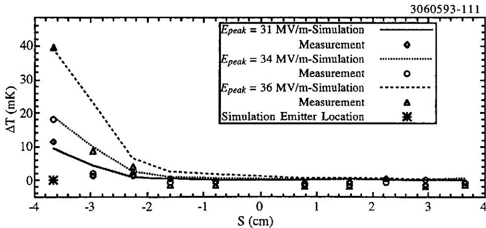
Figure 10. Comparison of measured and simulated temperature along board 8, in the final CW power rise.
