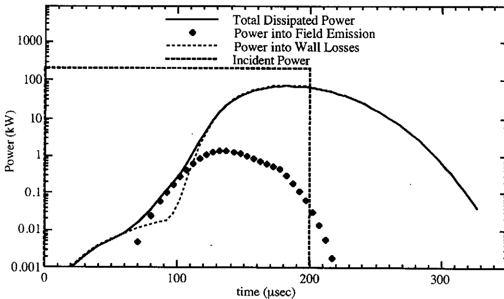
Figure 17. Power dissipation as a function of time during pulsed operation of a nine-cell cavity in quench conditions. Note that FE losses account for only 1% of total dissipation.
