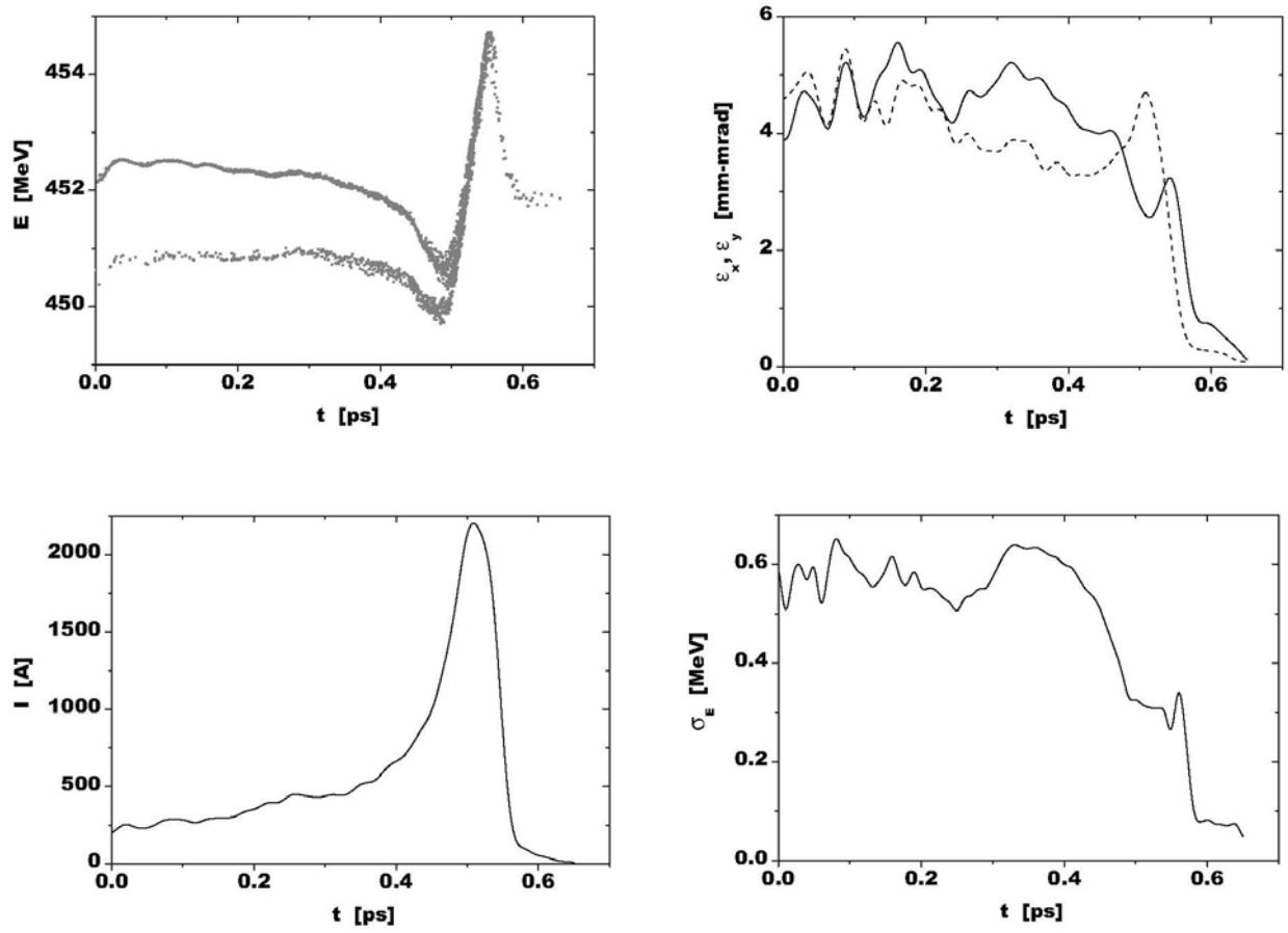
Figure 2: Longitudinal structure of a 1 nC electron bunch at the entrance of the undulator according to numerical beam dynamics simulation 21 . Top left: Local particle energy E . In the tail of the bunch, the energy distribution is broken in two branches. Bottom left: Current I . Top right: Normalized, transverse (“slice”) emittances \varepsilon_x (solid line) and \varepsilon_y (broken line). Bottom right: rms energy spread \sigma_E . All parameters are plotted as a function of the internal time variable t . The bunch head is to the right hand side.
