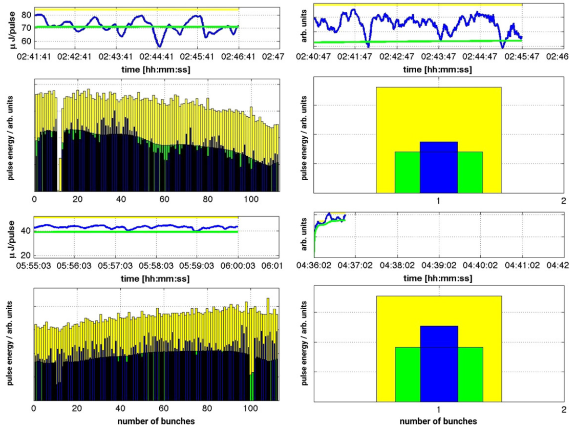
Figure 6. Lasing of the FLASH1 bunch train (left) and the one bunch at FLASH2 (right) for the charge parameters depicted in figure 5. Photon pulse energies of FLASH1 were measured using a GMD detector [20] with absolute calibration of the average signal and relative values for the individual pulses within the train. The pulse energy of FLASH2 was determined using an uncalibrated MCP detector [14]. For each pulse train instantaneous (blue), maximum (yellow) and average (green) pulse energies are shown.
