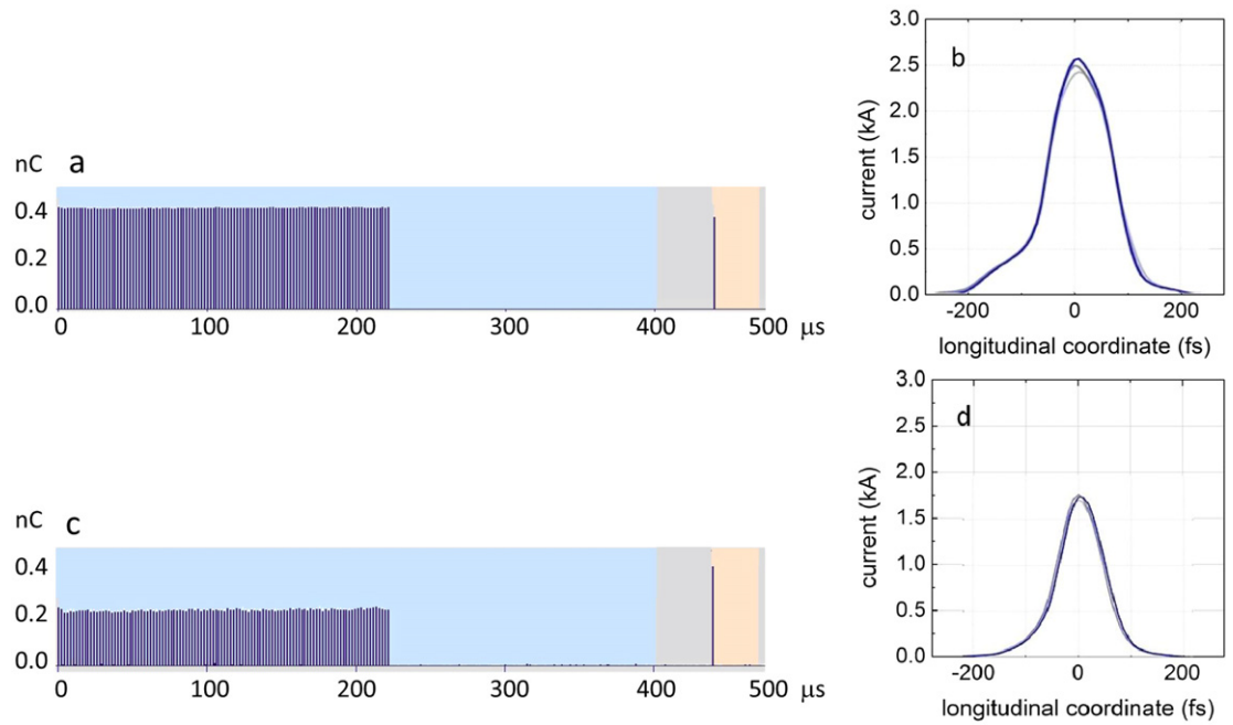
Figure 5. Two examples (a) and (c) of electron bunch trains with different charges for FLASH1 (blue section, 112 bunches) and for FLASH2 (orange section, 1 bunch). (b) and (d) show the corresponding peak currents measured for FLASH1. (b) has a bunch length of 75 fs (rms) and (d) has a bunch length of 50 fs (rms).
