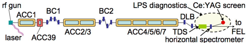
FIG. 2: (color online) Diagram of the FLASH facility. Only components affecting the longitudinal phase space beam (LPS) dynamics of the bunches are shown. The acronyms ACC, BC, and DBL stand respectively for accelerating modules, bunch compressors, and dogleg beamline (the blue rectangles represent dipole magnets). The transverse deflecting structure (TDS), spectrometer and Ce:YAG screen compose the LPS diagnostics.
