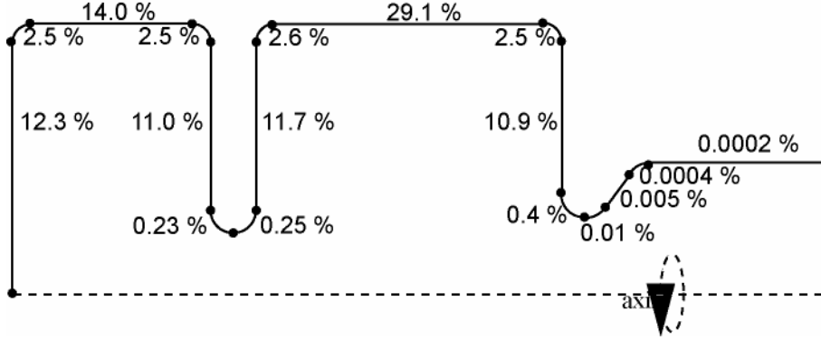
Figure 10: Relative power entries at specified wall segments around the rf-gun internal boundary as calculated with SUPERFISH.
